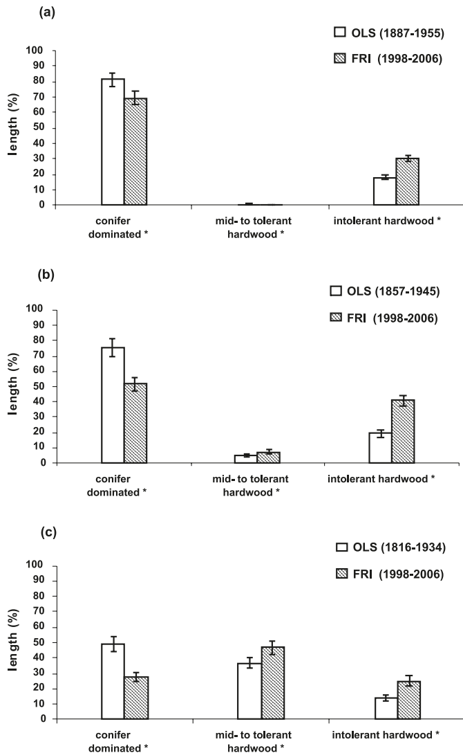
Fig. 2. Broad tree categories based on dominant species and logistic regression codes for birch for (a) SR3E, (b) SR4E, and (c) SR5E. Wilcoxon's signed ranks test was used to compare related proportions ( p < 0.001 for all samples).
